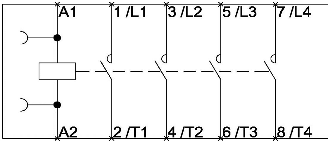
LEN00B004 Wiring Diagram
