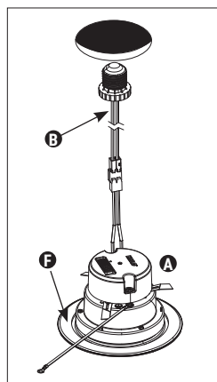
Figure 5 Retrofit
