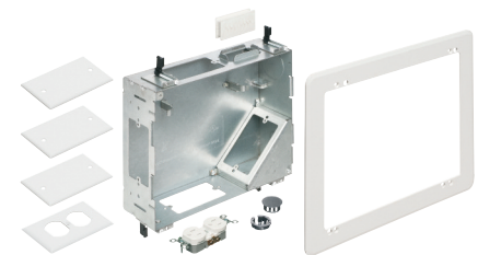
TVBS810 Components
