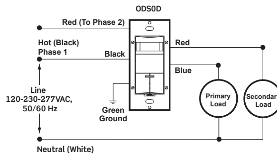
ODS0D-Ixx Wiring Diagram for Single Pole Application—2 Phase
