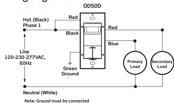
ODS0D-Ixx Wiring Diagram for Single Pole Application—Single Phase
