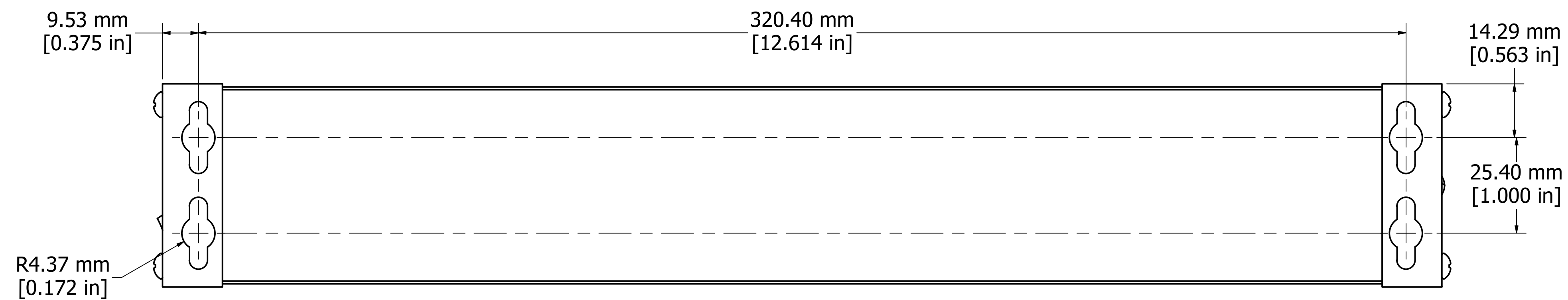
ASSEMBLY - VIEW FROM BOTTOM
