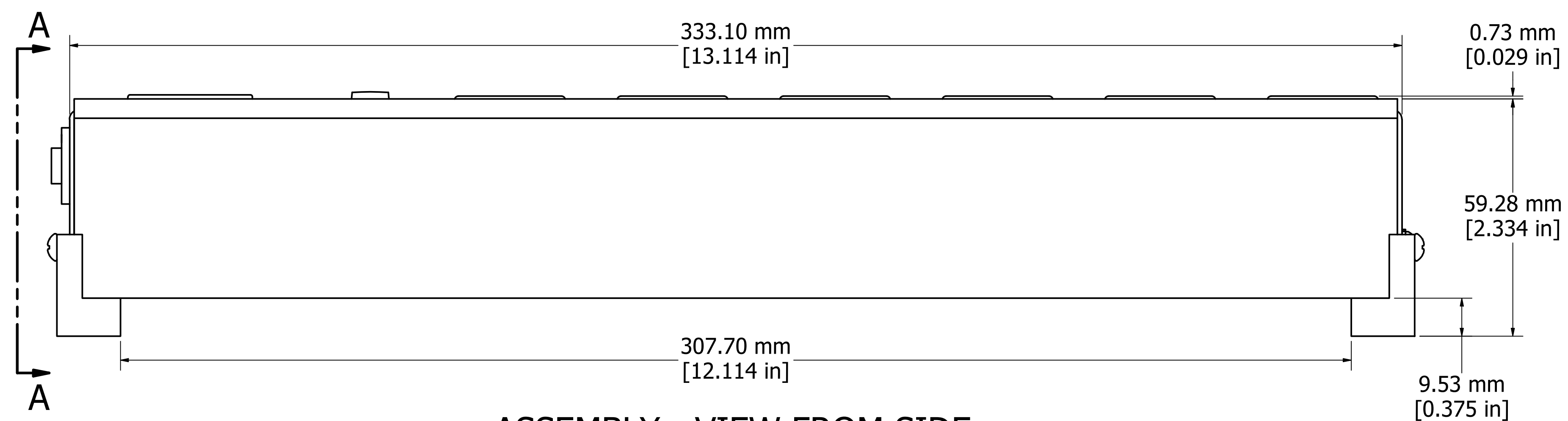
ASSEMBLY - VIEW FROM SIDE
