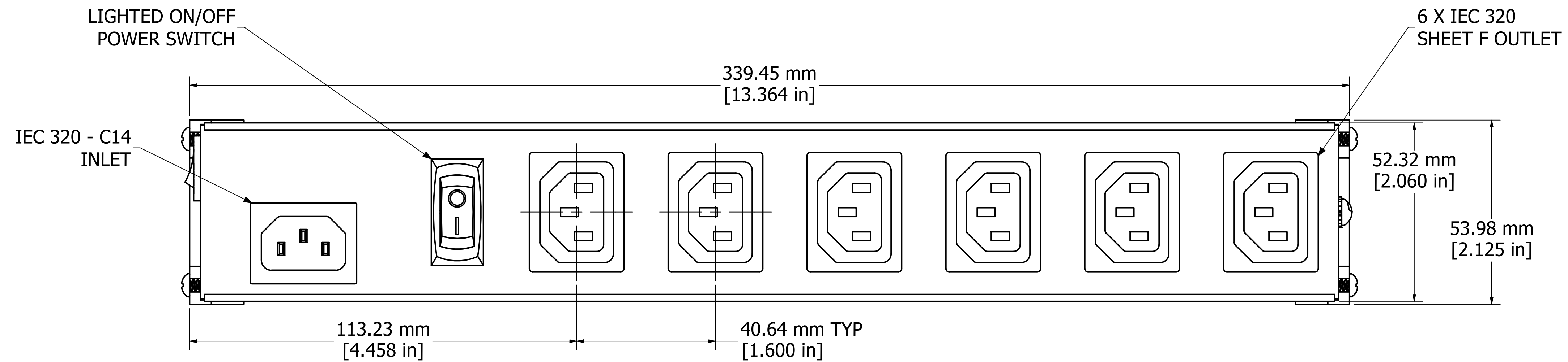
ASSEMBLY - VIEW FROM TOP
