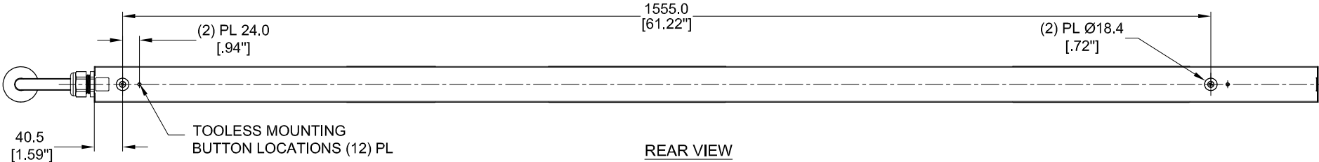
REAR VIEW
