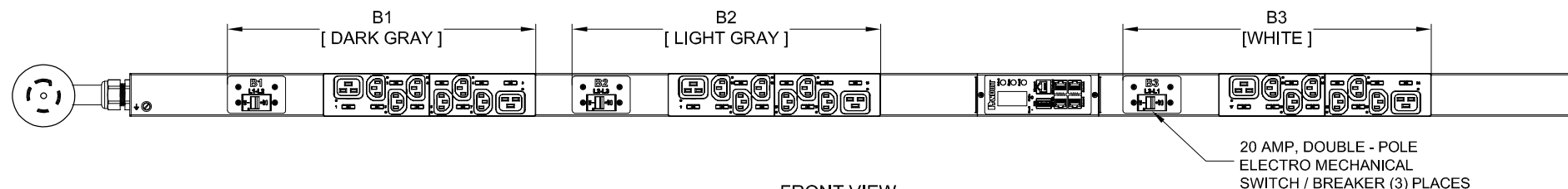
FRONT VIEW
