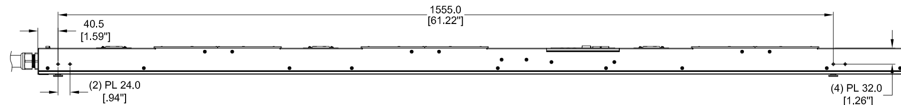
LEFT VIEW
