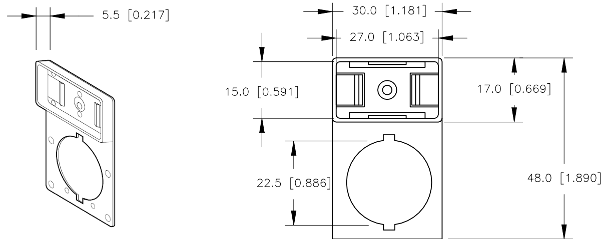
SELF ADHESIVE PUSH BUTTON MARKER HOLDER FOR TELEMECANIQUE OLD TYPE
