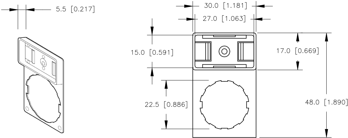
SELF ADHESIVE PUSH BUTTON MARKER HOLDER FOR TELEMECANIQUE HARMONY ZB4
