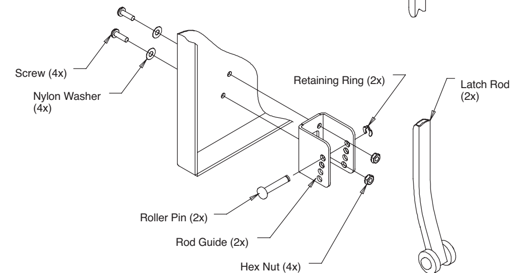
Latch Rod Assembly (Top and Bottom of Door)
