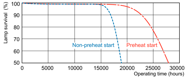
Life Expectancy Diagram - F54T5/850/HO/ALTO 40PK
