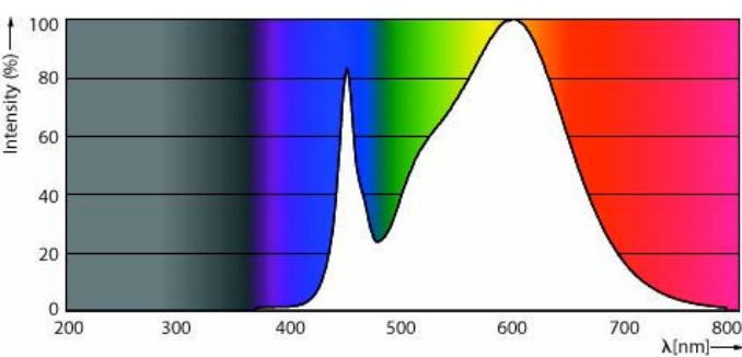
Spectral Power Distribution Colour - 17PL-L/COR/22-835/MF22/G/4P 10/1
