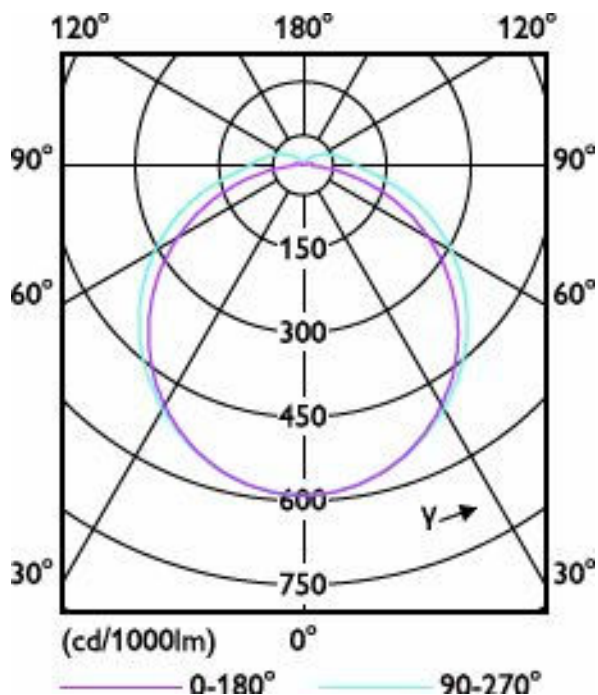
Light Distribution Diagram - 8PL-C/T/COR/26H-3CCT/MF10/P/20/1
