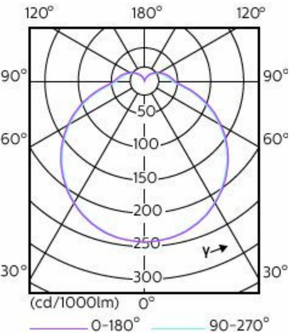
Light Distribution Diagram - 10.5PL-C/T/COR/26V-835/IF13/P/4P/DIM10/1
