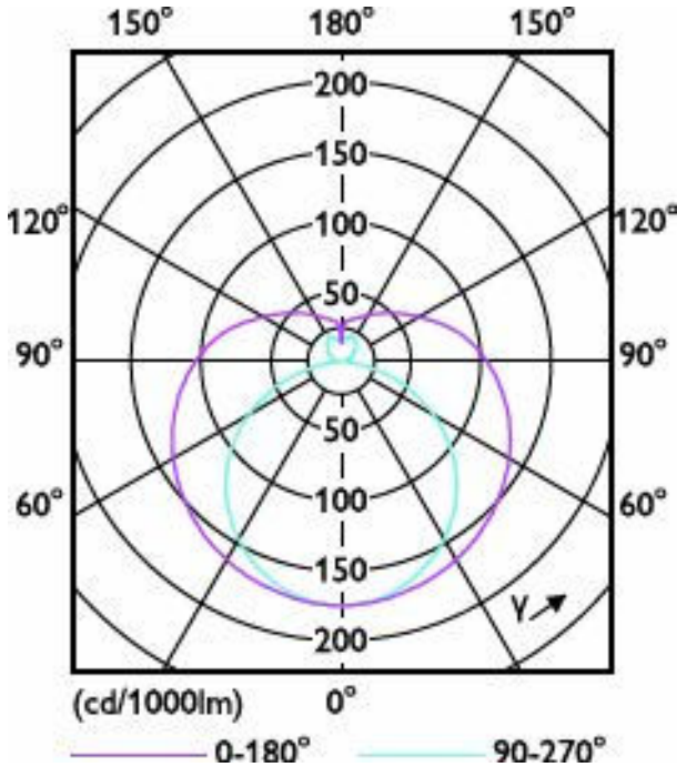
Light Distribution Diagram - 25T5HO/COR/46-850/MF35/G 25/1
