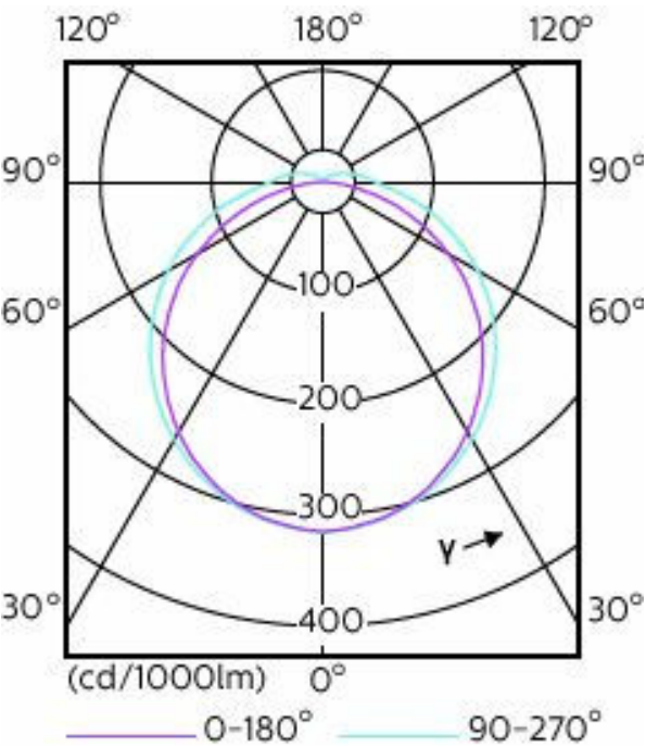
Light Distribution Diagram - 8.5PL-C/T/COR/ 26H-827/IF8/P/4P/DIM 10/1
