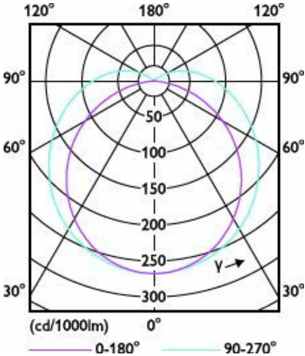
Light Distribution Diagram - 5.5PL-C/LED/13H/840/IF5/P/4P 20/1
