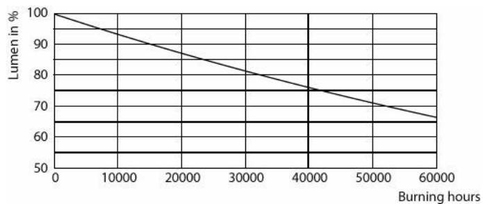
Lumen Maintenance Diagram - 5.5PL-C/LED/13H/840/IF5/P/4P 20/1
