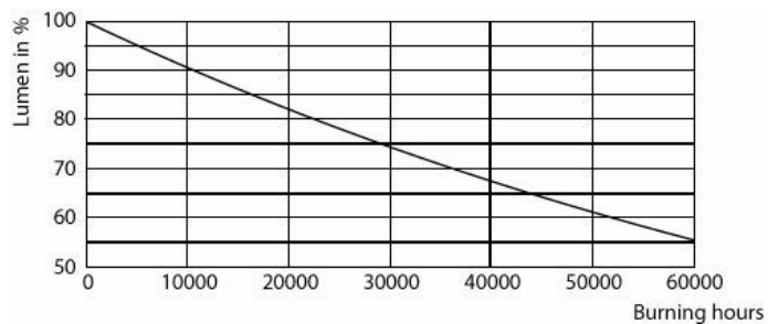
Lumen Maintenance Diagram - 11PL-C/T/COR/32V-3CCT/ MF15/P/20/1
