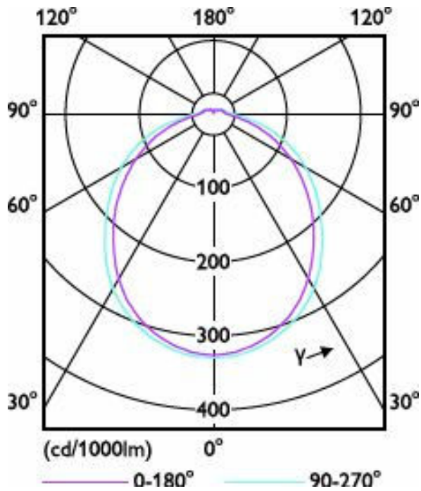
Light Distribution Diagram - 11PL-C/T/COR/32V-3CCT/MF15/P/20/1
