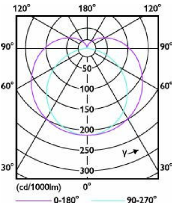
Light Distribution Diagram - 7T8/MAS/24-850/IF11/P/DIM 10/1
