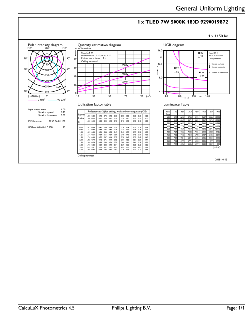
General uniform lighting - 7T8/MAS/24-850/IF11/P/DIM 10/1
