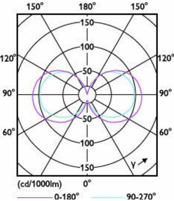
Light Distribution Diagram - 5.5B11/PER/927-922/CL/G/E26/WGX 1FB T20
