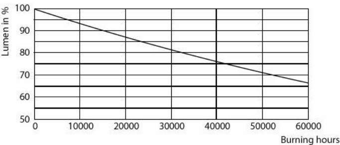
Lumen Maintenance Diagram - 150CC/MAS/840/LS EX39 G2 BB 3/1
