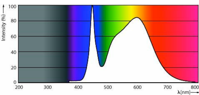
Spectral Power Distribution Colour - 150CC/MAS/840/LS EX39 G2 BB 3/1
