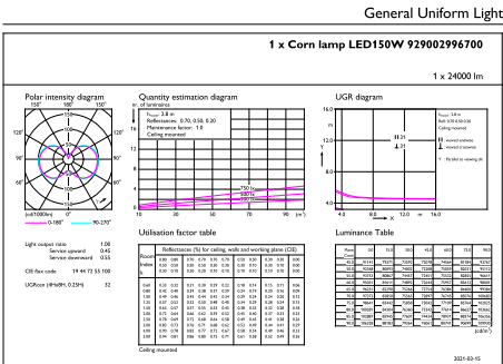
Light Distribution Diagram - 150CC/MAS/840/LS EX39 G2 BB 3/1
