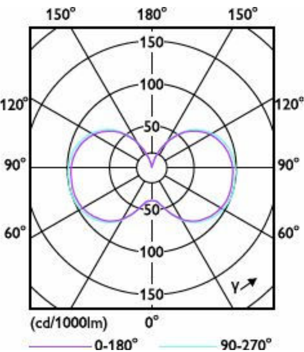
Light Distribution Diagram - 150CC/MAS/840/LS EX39 G2 BB 3/1
