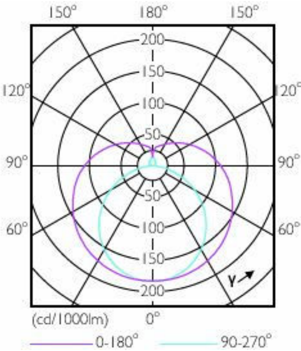
Light Distribution Diagram - 11T5HE/34-840/IF15/G/DIM 10/1
