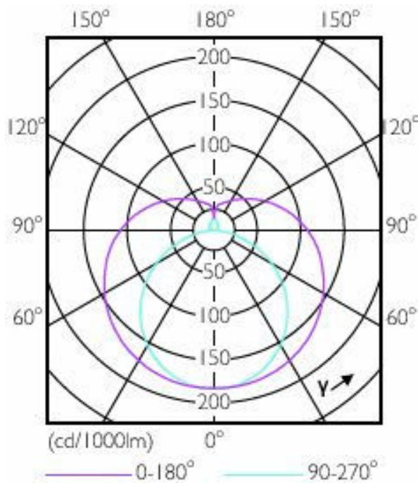
Light Distribution Diagram - 8T5HE/22-835/IF10/G/DIM 10/1
