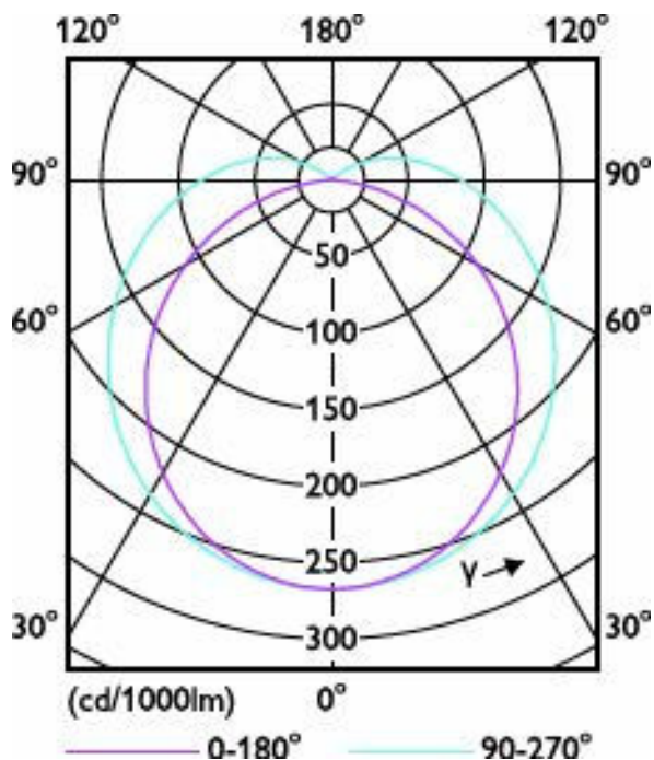
Light Distribution Diagram - 5.5PL-C/LED/13H/835/IF5/P/4P 20/1
