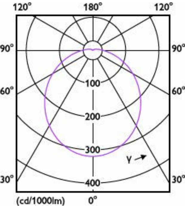
Light Distribution Diagram - 7.2BR30/COR/930/P/E26/DIM 6/1FB T20
