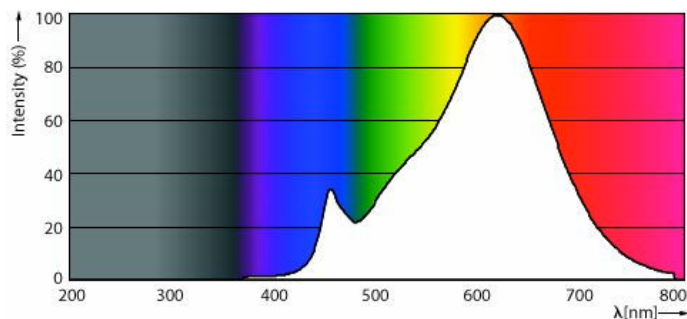
Spectral Power Distribution Colour - 3.3B11/PER/ 927-922/CL/G/E12/WGX 1FB T20
