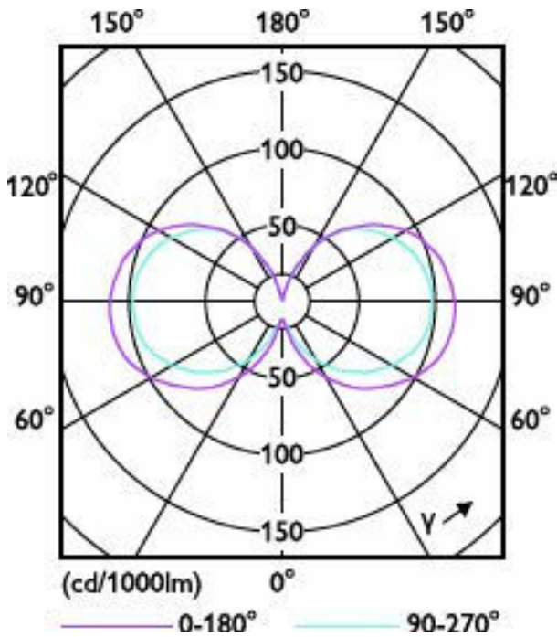
Light Distribution Diagram - 3.3B11/PER/927-922/CL/G/E12/WGX 1FB T20
