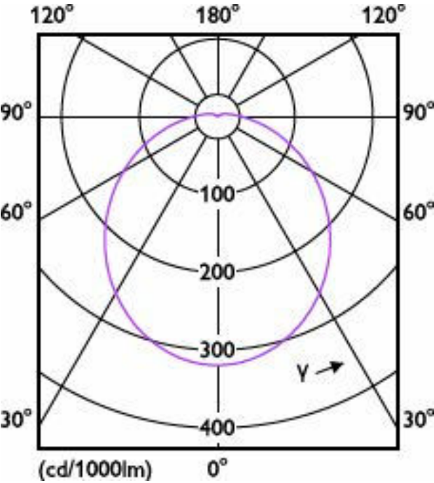
Light Distribution Diagram - 7.2BR30/COR/940/P/E26/DIM 6/1FB T20
