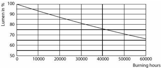
Lumen Maintenance Diagram - 12PL-C/T/COR/32H-835/ IF14/P/4P/DIM 10/1
