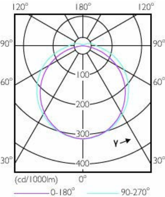
Light Distribution Diagram - 12PL-C/T/COR/32H-835/ IF14/P/4P/DIM 10/1
