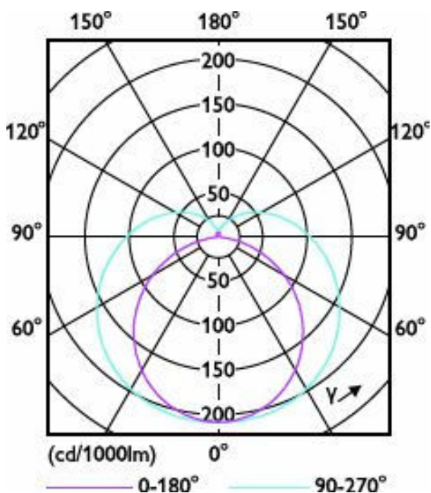
Light Distribution Diagram - 15.5T8/MAS/48-840/IF25/P/DIM 25/1
