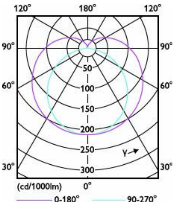
Light Distribution Diagram - 8.5T8/MAS/36-835/IF13/P/DIM 10/1
