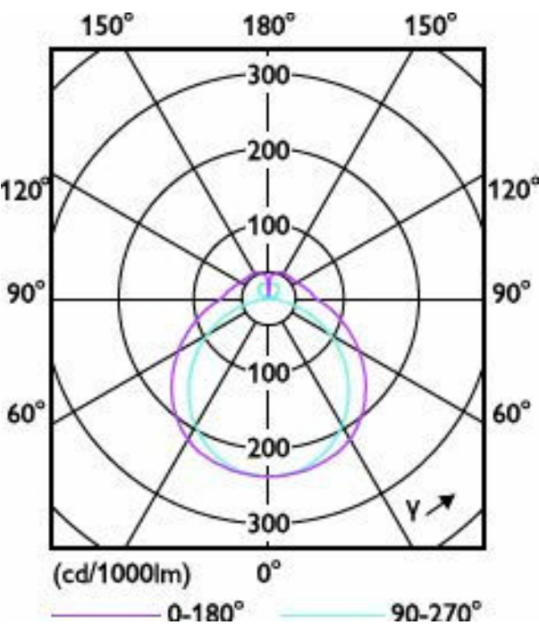
Light Distribution Diagram - 17PL-L/COR/22-840/MF22/G/4P 10/1
