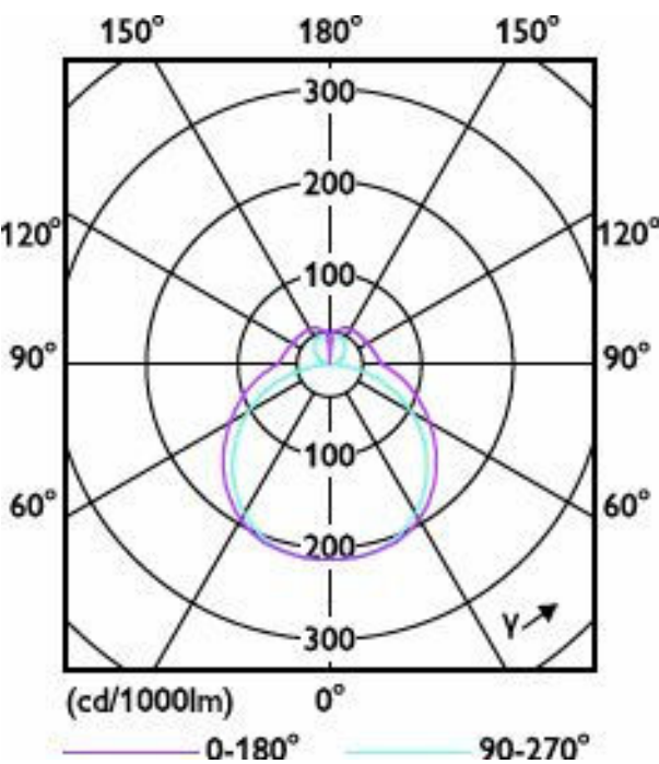
Light Distribution Diagram - 17PL-L/COR/22-835/MF22/G/4P 10/1
