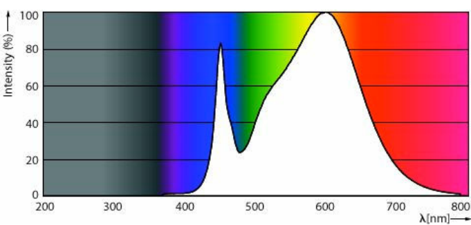
Spectral Power Distribution Colour - 17PL-L/COR/22-835/MF22/G/4P 10/1
