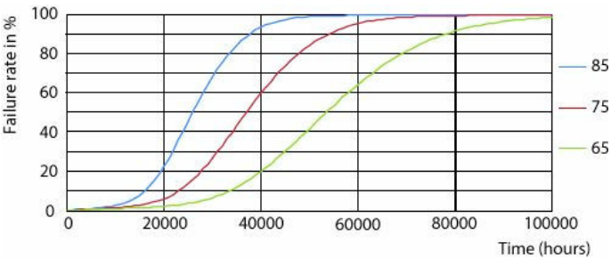
LEDtube COR PLL 17W 50K FailureRate-LED
