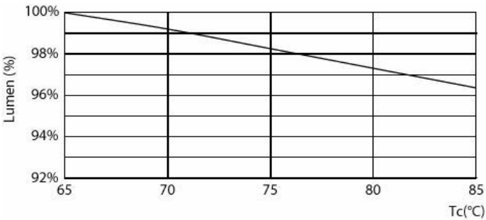
Lumen Maintenance Diagram - 17PL-L/COR/22-835/MF22/G/4P 10/1
