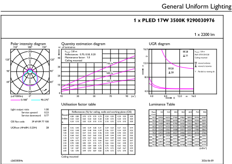
Light Distribution Diagram - 17PL-L/COR/22-835/MF22/G/4P 10/1
