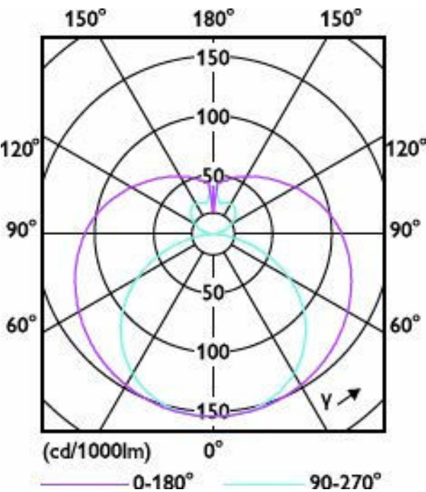
Light Distribution Diagram - 14.5T8/COR/48-850/MF21/G/DIM 25/1
