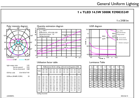
Light Distribution Diagram - 14.5T8/COR/48-850/MF21/G/DIM 25/1
