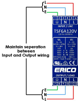
Figure 1: Wiring Diagram
