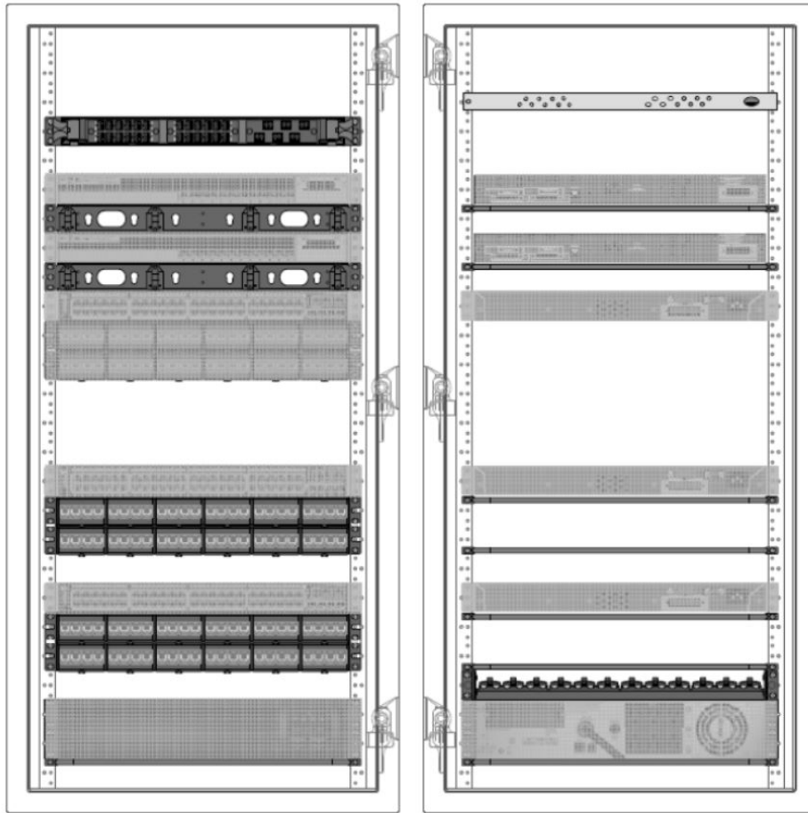
Front View
