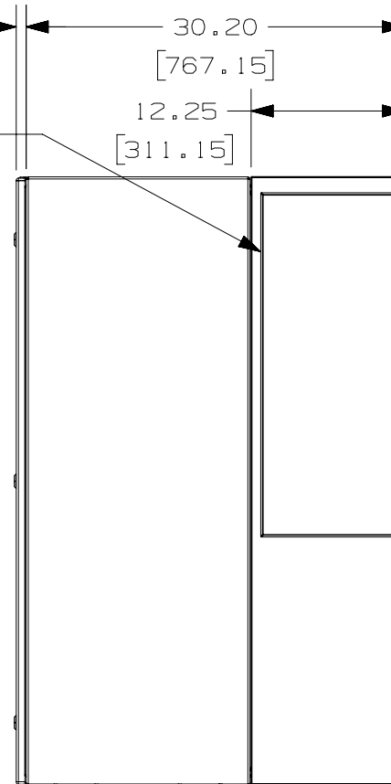
SIDE VIEW
