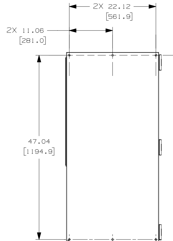
BACK VIEW
