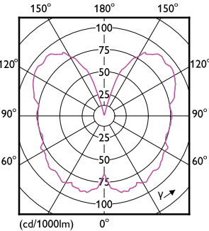
Light Distribution Diagram - 5.5ST19/VIN/927/E26/CL/G/SP D 1PF T20
