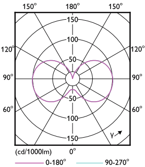
Light Distribution Diagram - 450CC/LED/840/LS EX39 BB 3/1
