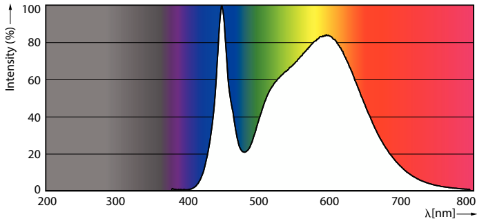
Spectral Power Distribution Colour - 450CC/LED/840/LS EX39 BB 3/1
