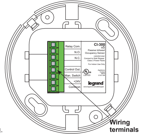
Manual-On wiring with low voltage momentary switch
